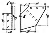
Figs. 4173-4174. Tank Cover Brace Plate.
